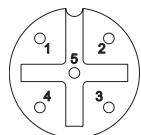
plug soldered side
